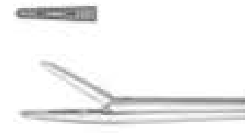
12-111 Hartmann shaft length 85 mm
