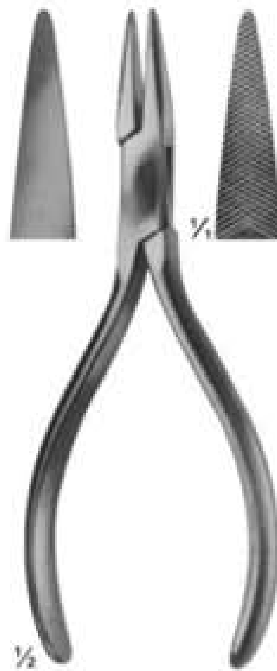
17-196 one jaw smooth, one jaw serrated 140 mm
